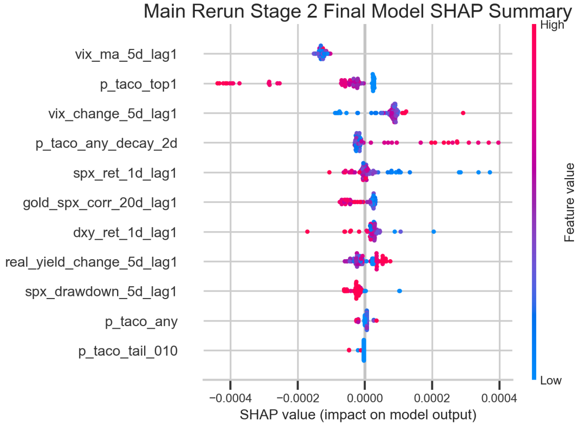
Figure 2: Appendix Figure A1. SHAP summary for the selected Stage 2 two-stage model on the holdout sample.
